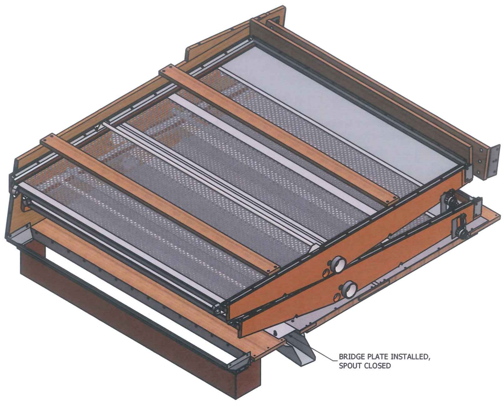
RIGHT SIDE CUTAWAY, BOTTOM ROCKER SCALP FLOW ARRANGEMENT SCALE 1/8 BOTTOM ROCKER SHOWN AT MINIMUM PITCH
