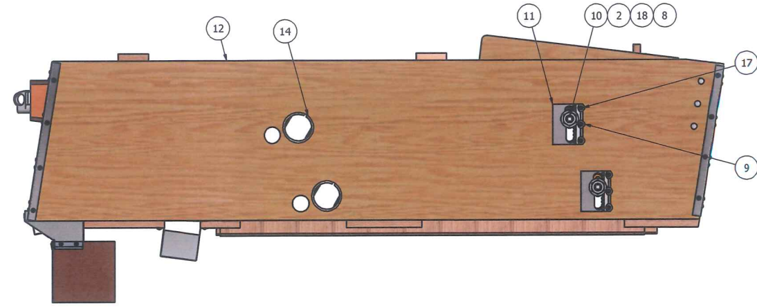
STEP 2: RIGHT SIDE VIEW, TOP ROCKER INSTALLATION
