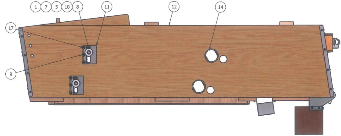
LEFT SIDE VIEW, TOP ROCKER INSTALLATION
