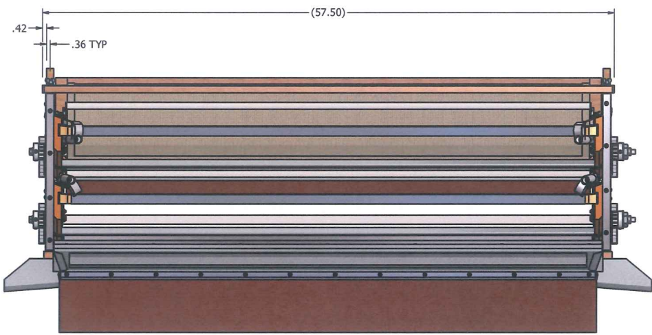
RIGHT SIDE CUTAWAY, BOTTOM ROCKER SCALP FLOW ARRANGEMENT SCALE 1/8 BOTTOM ROCKER SHOWN AT MINIMUM PITCH
