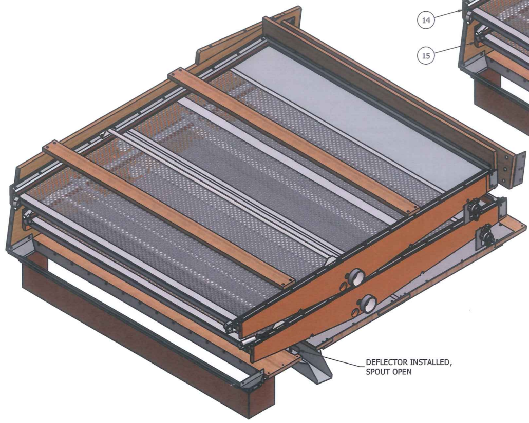
RIGHT SIDE CUTAWAY, BOTTOM ROCKER SIFT FLOW ARRANGEMENT SCALE 1/8 TOP ROCKER SHOWN AT MAXIMUM PITCH
