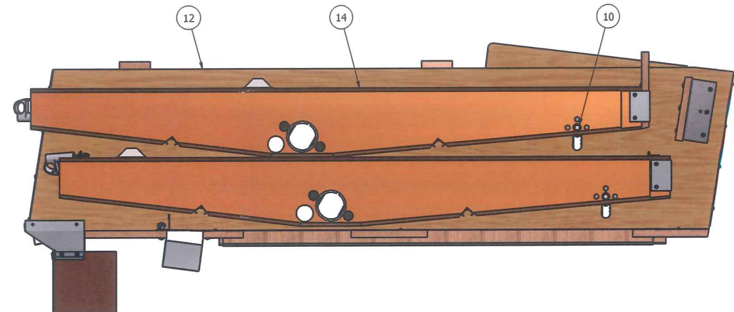
RIGHT SIDE CUTAWAY
