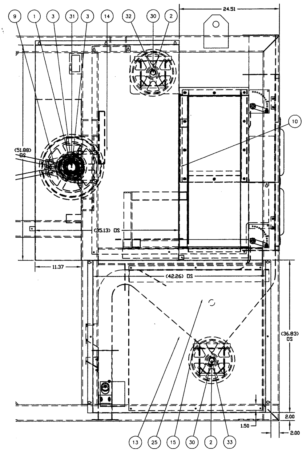
RIGHT SIDE VIEW REAR DETAIL
