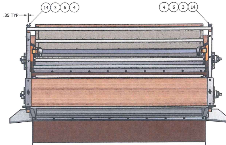
RIGHT SIDE CUTAWAY, DEFLECTOR INSTLLED SCALE 1/8
