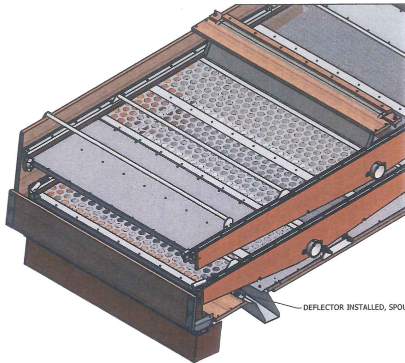
RIGHT SIDE CUTAWAY, DEFLECTOR INSTLLED SCALE 1/8
