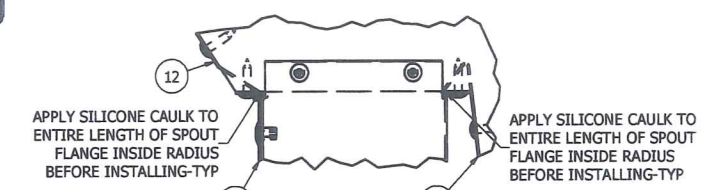
DETAIL D SCALE 1 / 2
