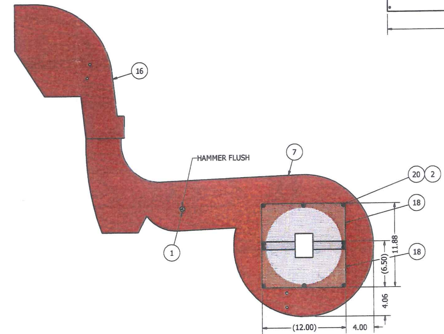
STEP #2-LOWER WRAPPER ASSEMBLY
