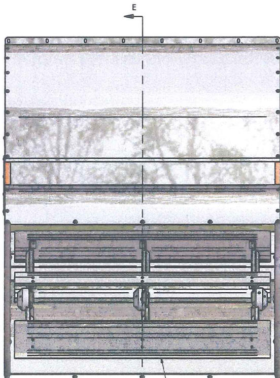
STEP #7-FAN INSTALLATION, FRONT VIEW
