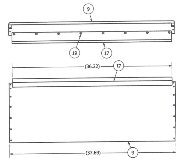
STEP #2-LOWER WRAPPER ASSEMBLY
