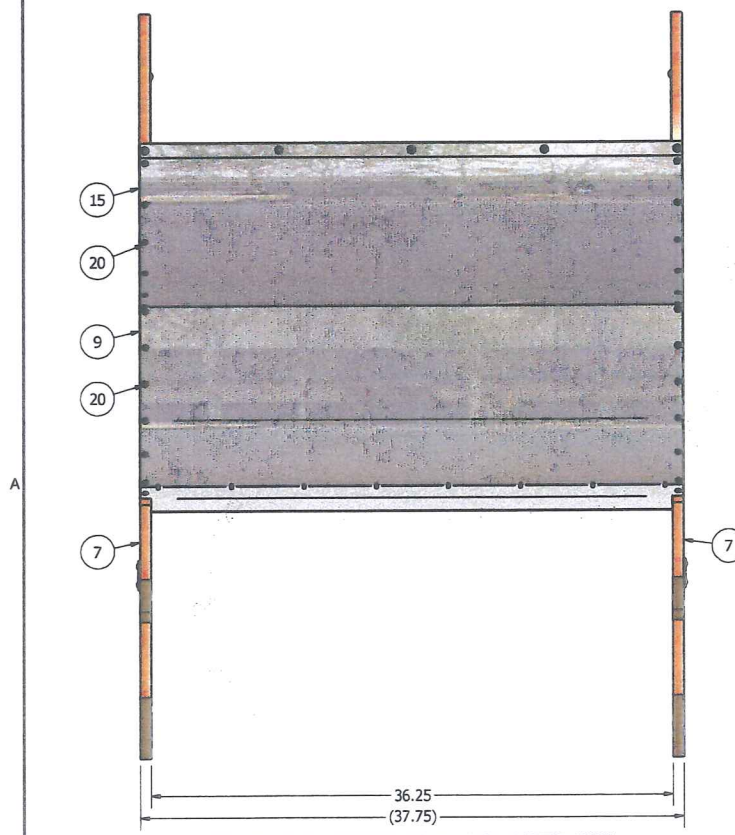
STEP #3-LOWER WRAPPER INSTALLATION, BOTTOM VIEW
