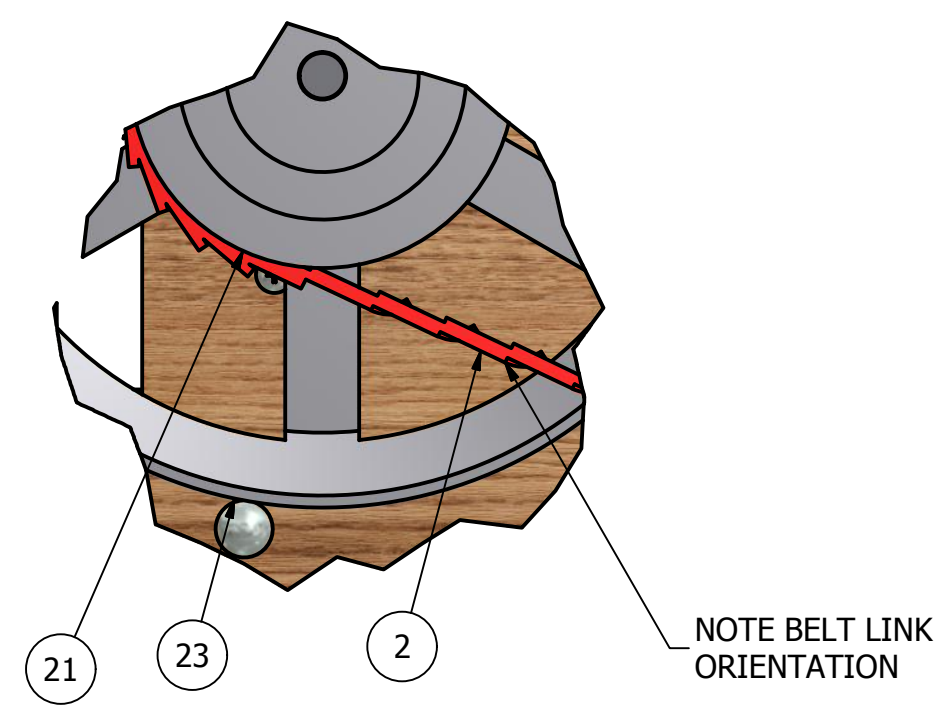
DETAIL A SCALE 1/2
